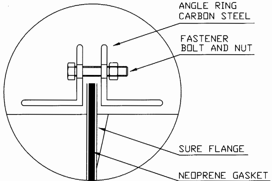
COMPANION FLANGE DETAIL
